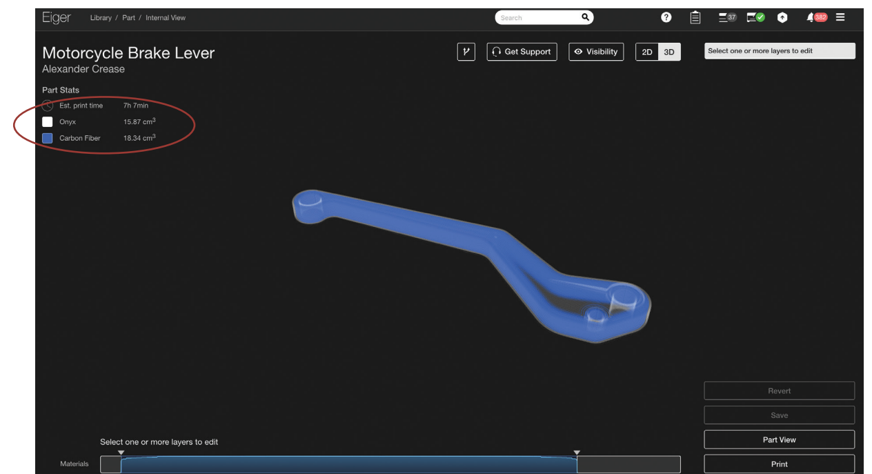
The internal view of our motorcycle brake lever sample part.
